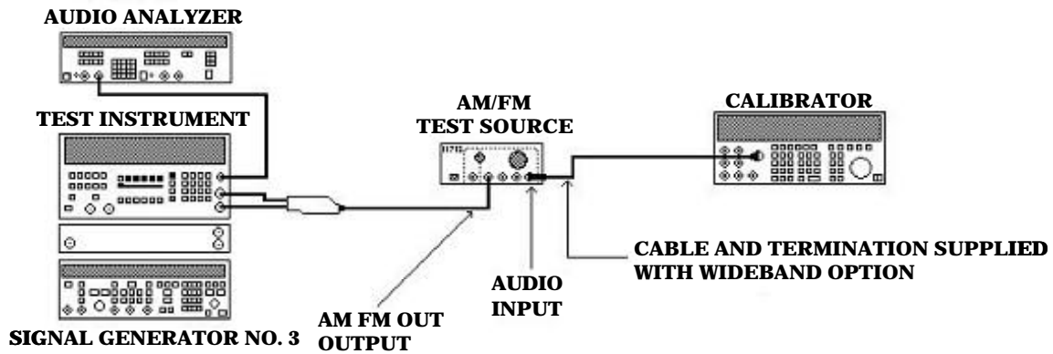
Figure 11. Phase modulation setup.
